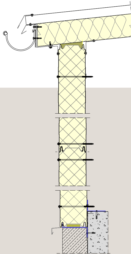
Principle detail of facade
