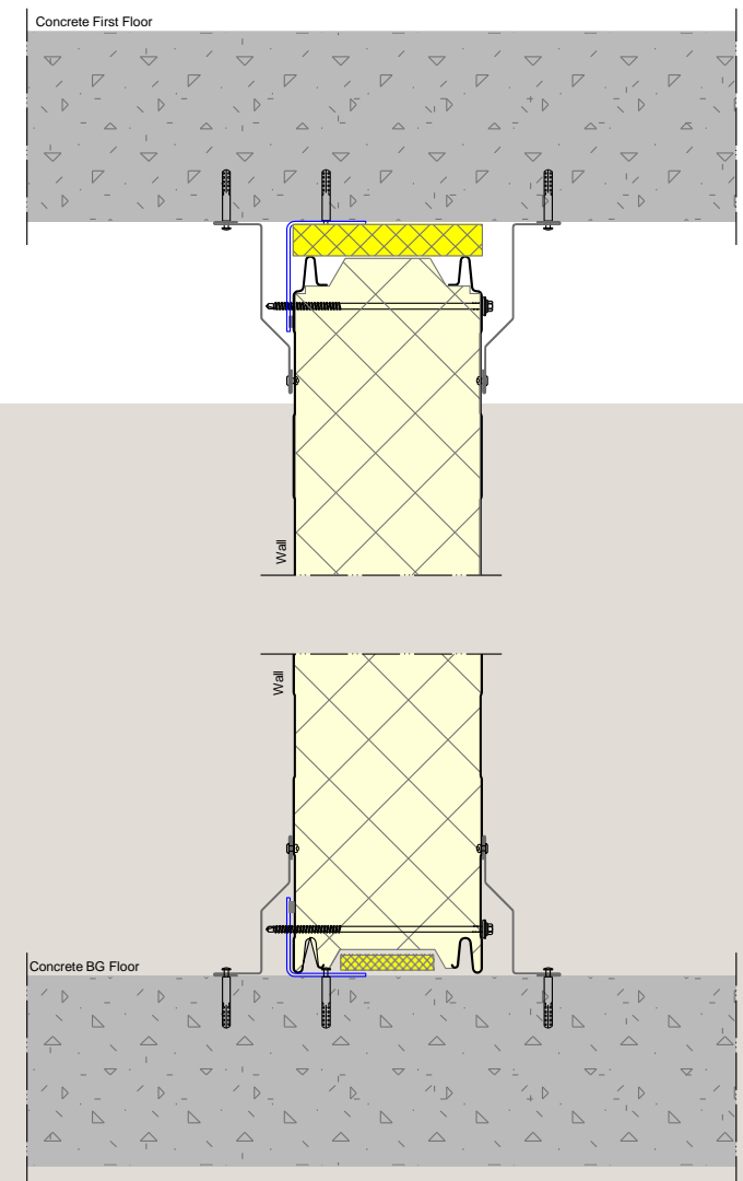
Principle detail of partition wall
